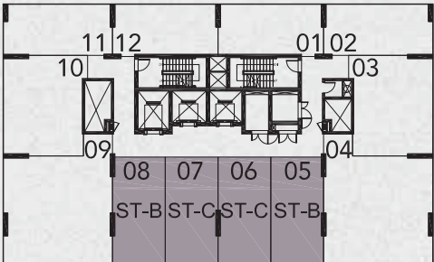
LEVEL 10-16
